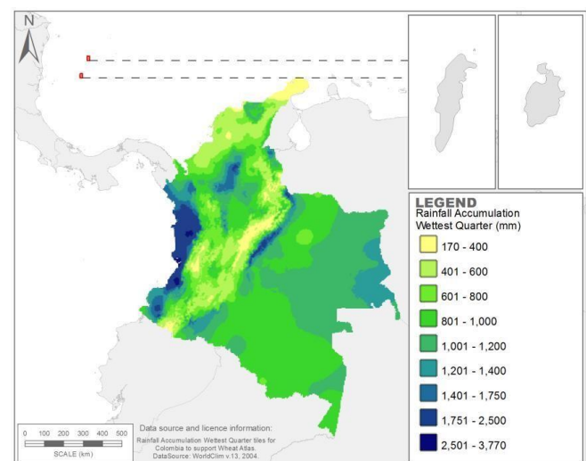
Fig. 1. Precipitation
